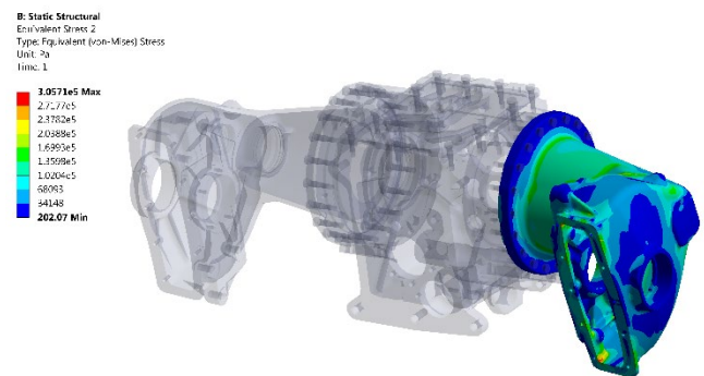
Stress distribution in an axle, courtesy of ANSYS Corp
